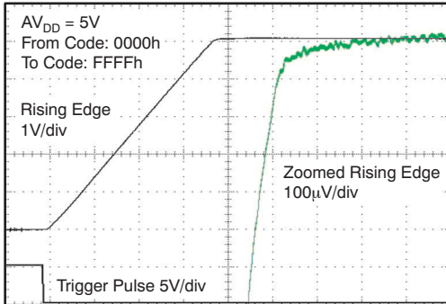
FULL-SCALE SETTLING TIME 5V RISING EDGE
