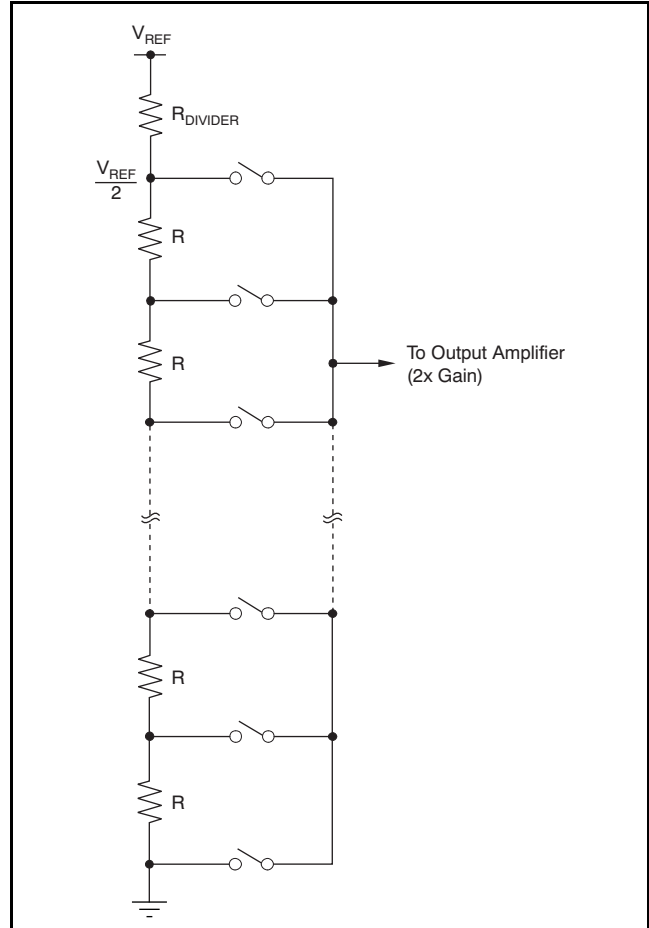
Figure 93. Resistor String
