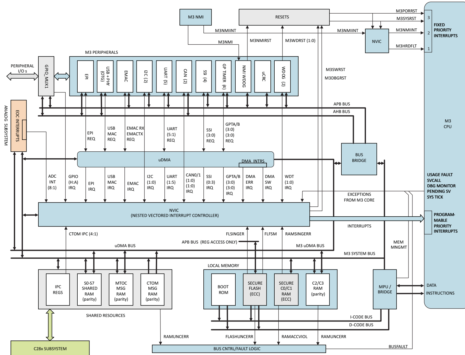
Figure 2-1. Master Subsystem
