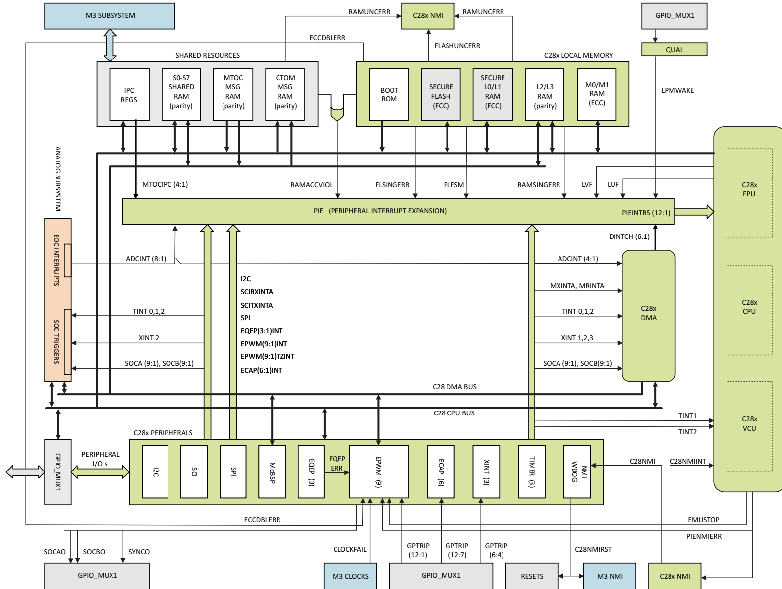
Figure 2-2. Control Subsystem
