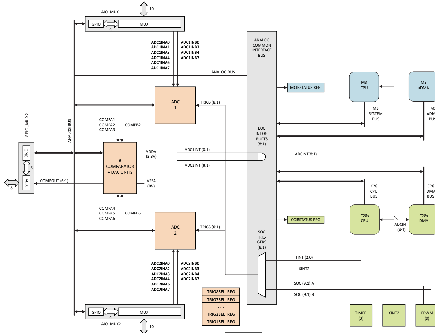
Figure 2-3. Analog Subsystem
