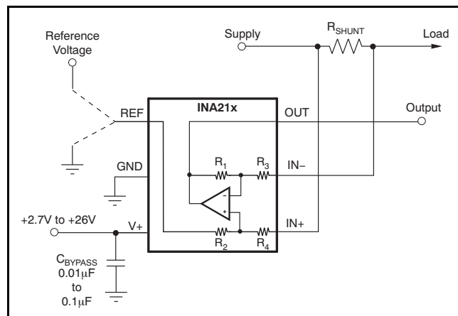
Figure 23. Typical Application
