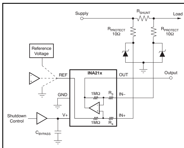
Figure 27. INA210-INA214 Transient Protection Using Dual Zener Diodes
