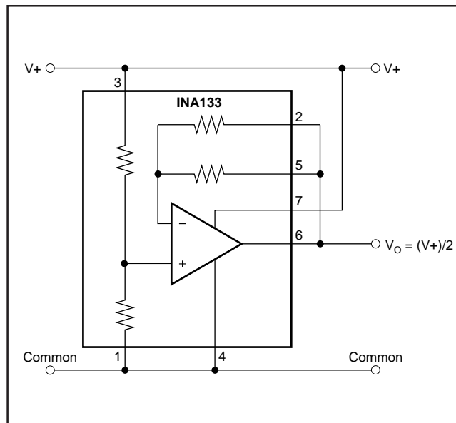
FIGURE 5. Pseudoground Generator.
