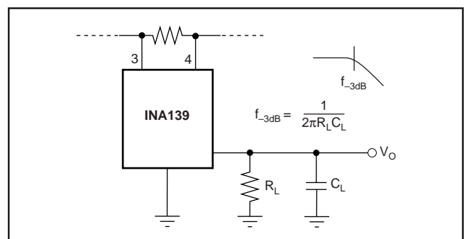
FIGURE 3. Output Filter.
