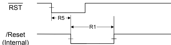
Figure 22-6. External Reset Timing ( \overline{RST} )
