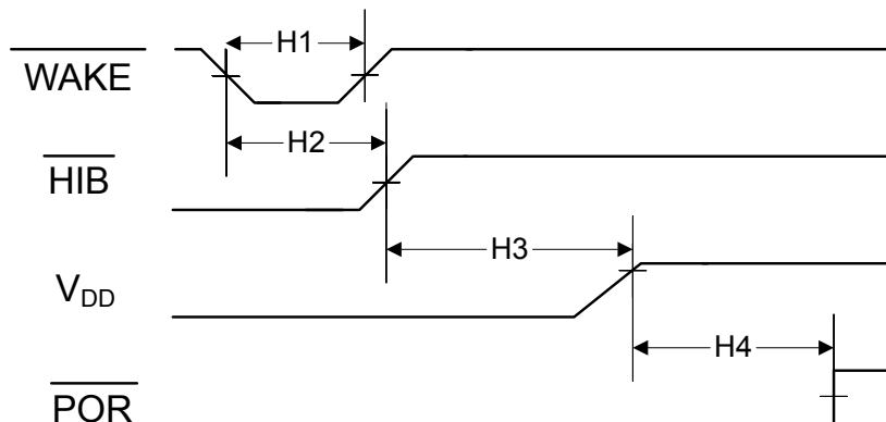
Figure 22-10. Hibernation Module Timing
