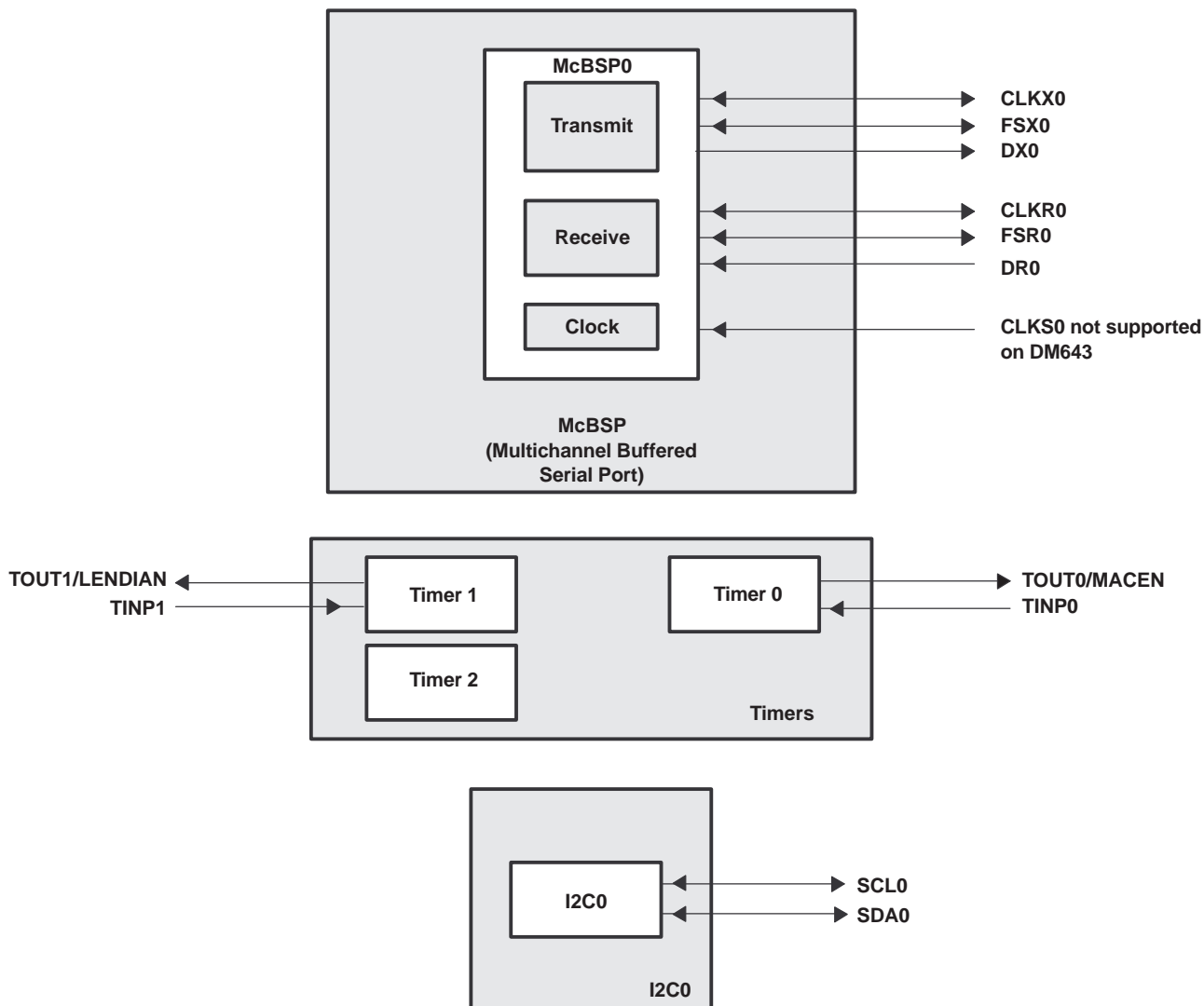
Figure 2-10. McBSP/Timer/I2C0 Peripheral Signals
