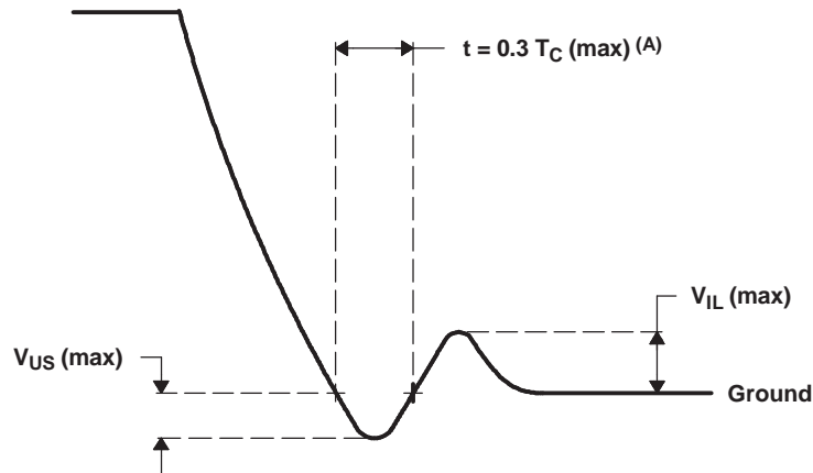
Figure 5-5. AC Transient Specification Fall Time
