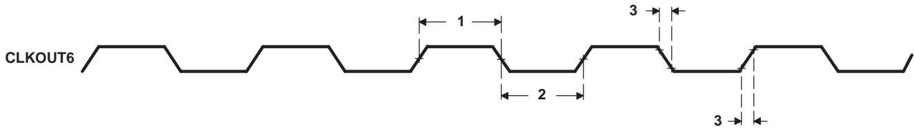
Figure 5-15. CLKOUT6 Timing
