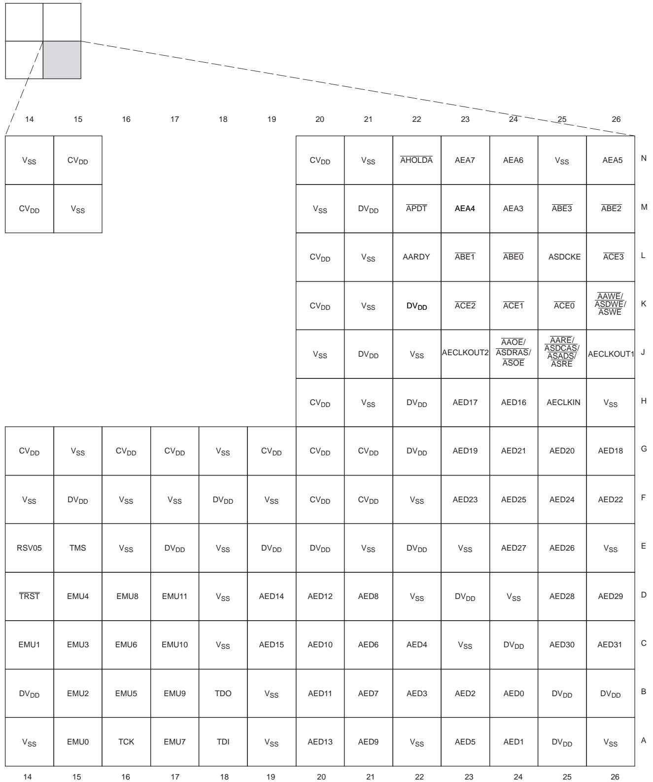
Figure 2-6. DM643 Pin Map [Quadrant D]
