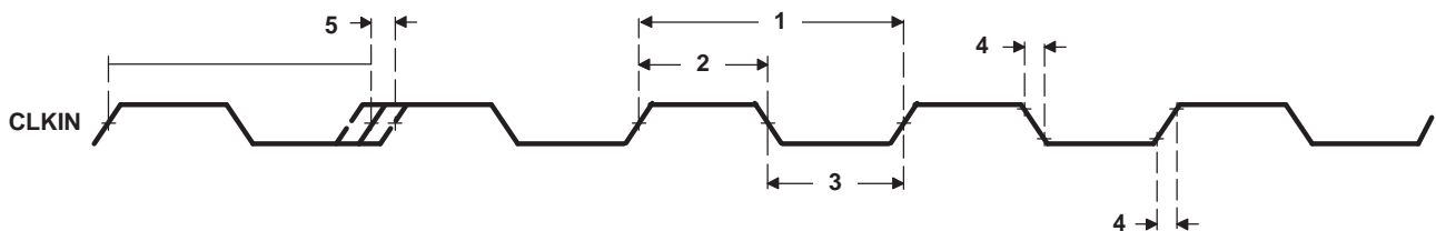
Figure 5-13. CLKIN Timing
