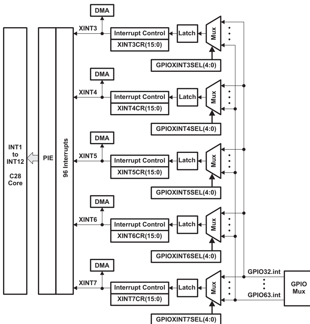
Figure 3-6. External Interrupts
