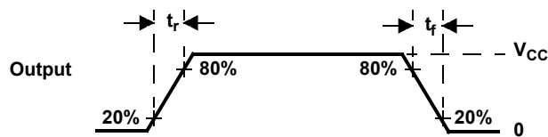
Figure 9. CMOS-Level Outputs
