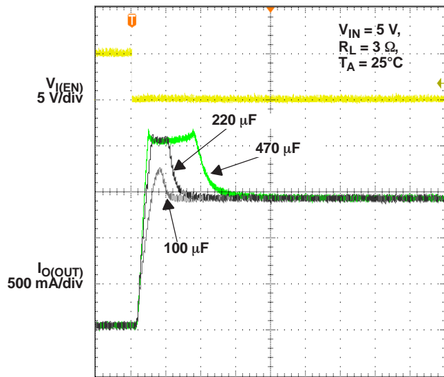
t - Time - 500 \mu\text{s}/\text{div}
