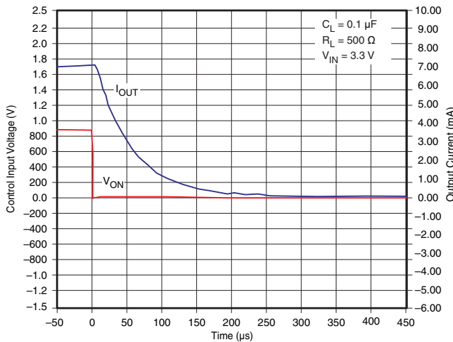
Figure 26. t_{OFF} Response
