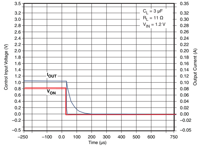
Figure 57. t OFF Response
