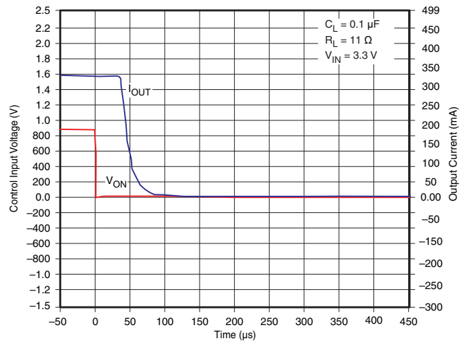
Figure 27. t_{OFF} Response
