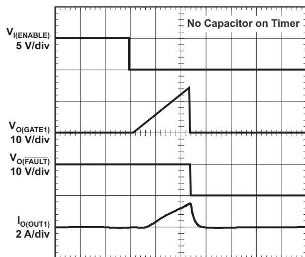
Figure 5. Channel 1 Overcurrent Response: Enabled Into Overcurrent Load
