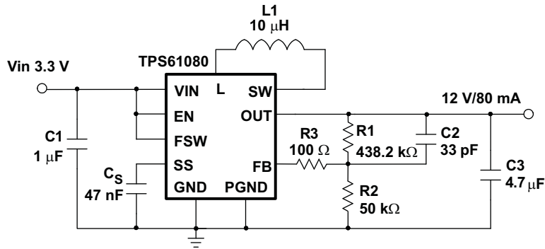
L1: Sumida CDRH4D16FBNP-100NC C1: Murata GRM188R60J105K; C3: Murata GRM219R61C475K
