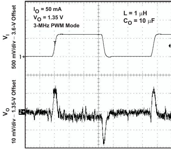
LINE TRANSIENT PWM OPERATION
