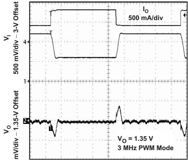
COMBINED LINE/LOAD TRANSIENT (3.6 V TO 4.2 V, 400 mA TO 800 mA) PWM OPERATION
