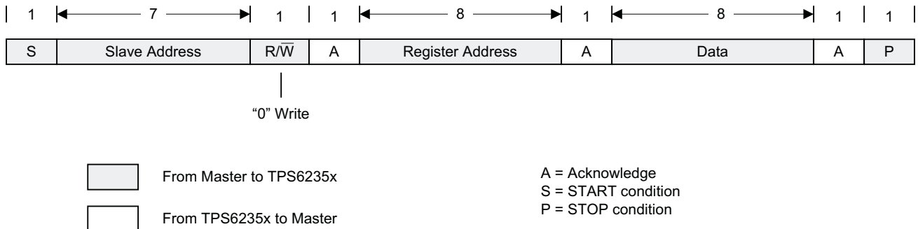
Figure 49. "Write" Data Transfer Format in F/S-Mode
