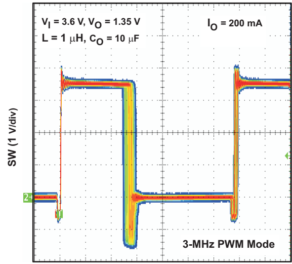
DUTY CYCLE JITTER
