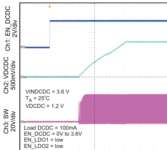
STARTUP TIMING (DCDC)
