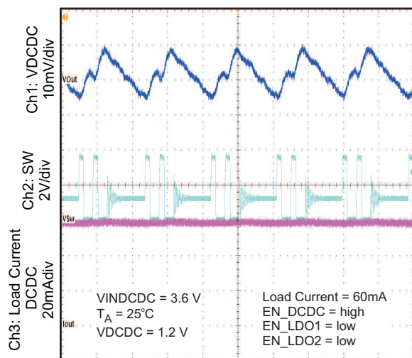
OUTPUT VOLTAGE RIPPLE (DCDC PFM Mode)
