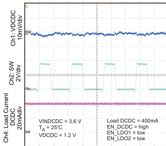
OUTPUT VOLTAGE RIPPLE (DCDC PWM Mode)
