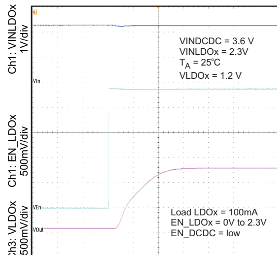
START-UP TIMING (LDOx)
