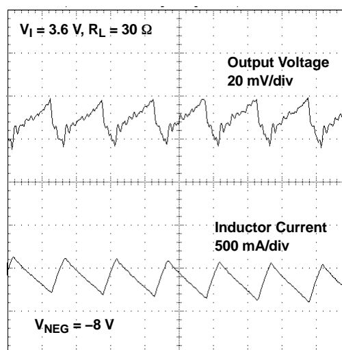
NEGATIVE OUTPUT VOLTAGE IN CONTINUOUS CURRENT MODE
