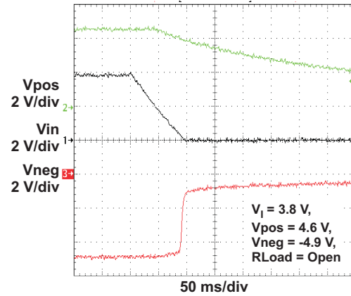
Figure 12. SHUTDOWN
