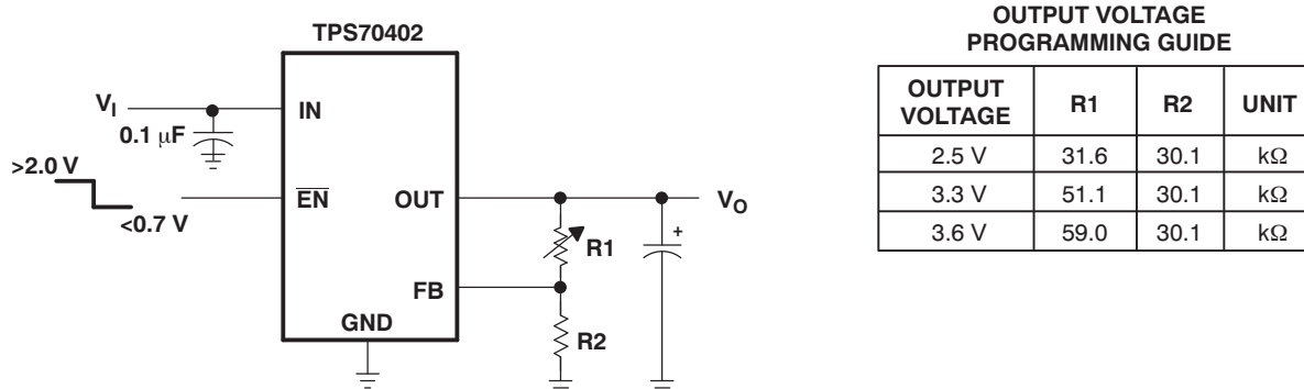
Figure 41. TPS70402 Adjustable LDO Regulator Programming
