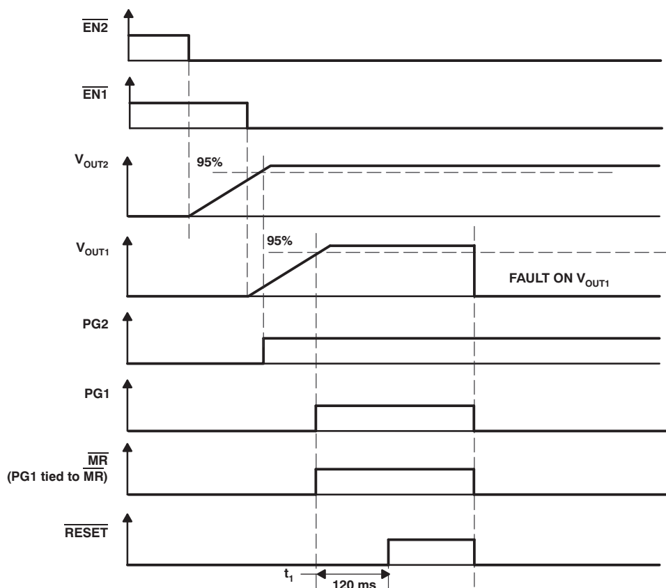
Figure 40. Timing When There is a Fault on V_{OUT1}
