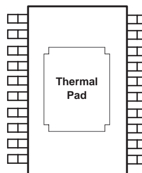
PWP PACKAGE (BOTTOM VIEW)
