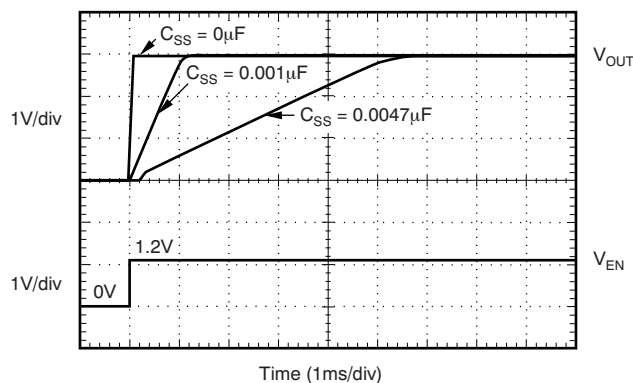
Figure 1. Turn-On Response
