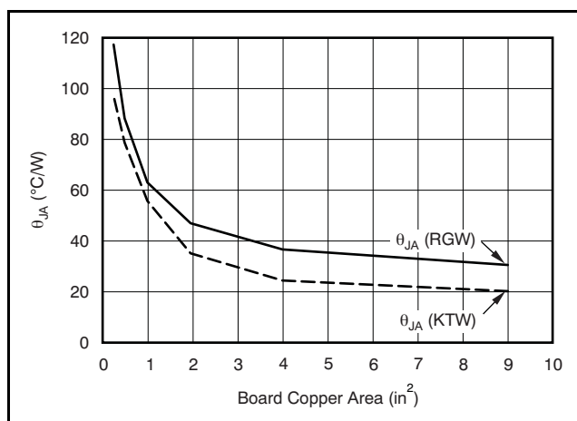
Figure 33. \theta_{JA} vs Board Size
