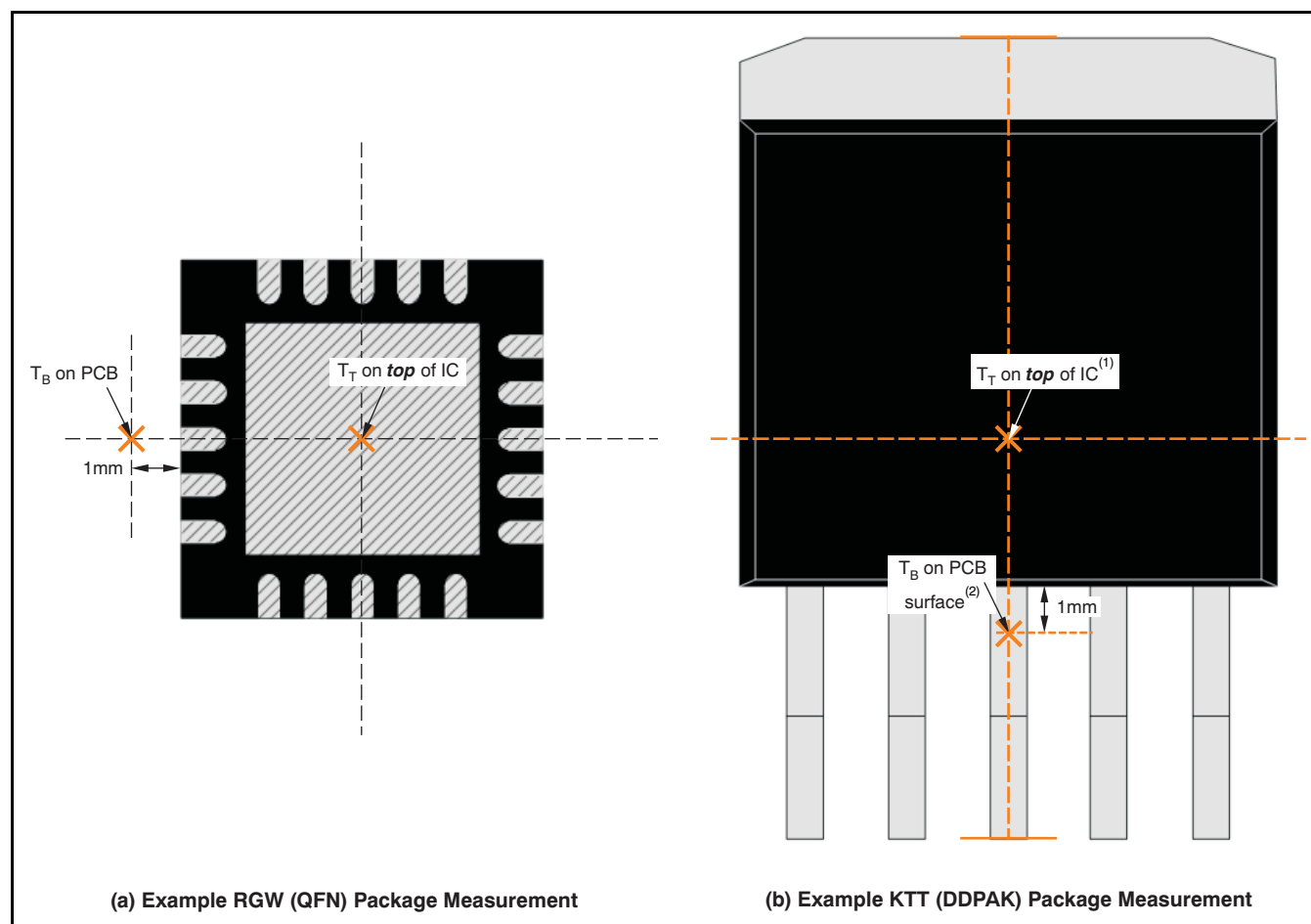
Figure 34. Measuring Point for T_T and T_B
