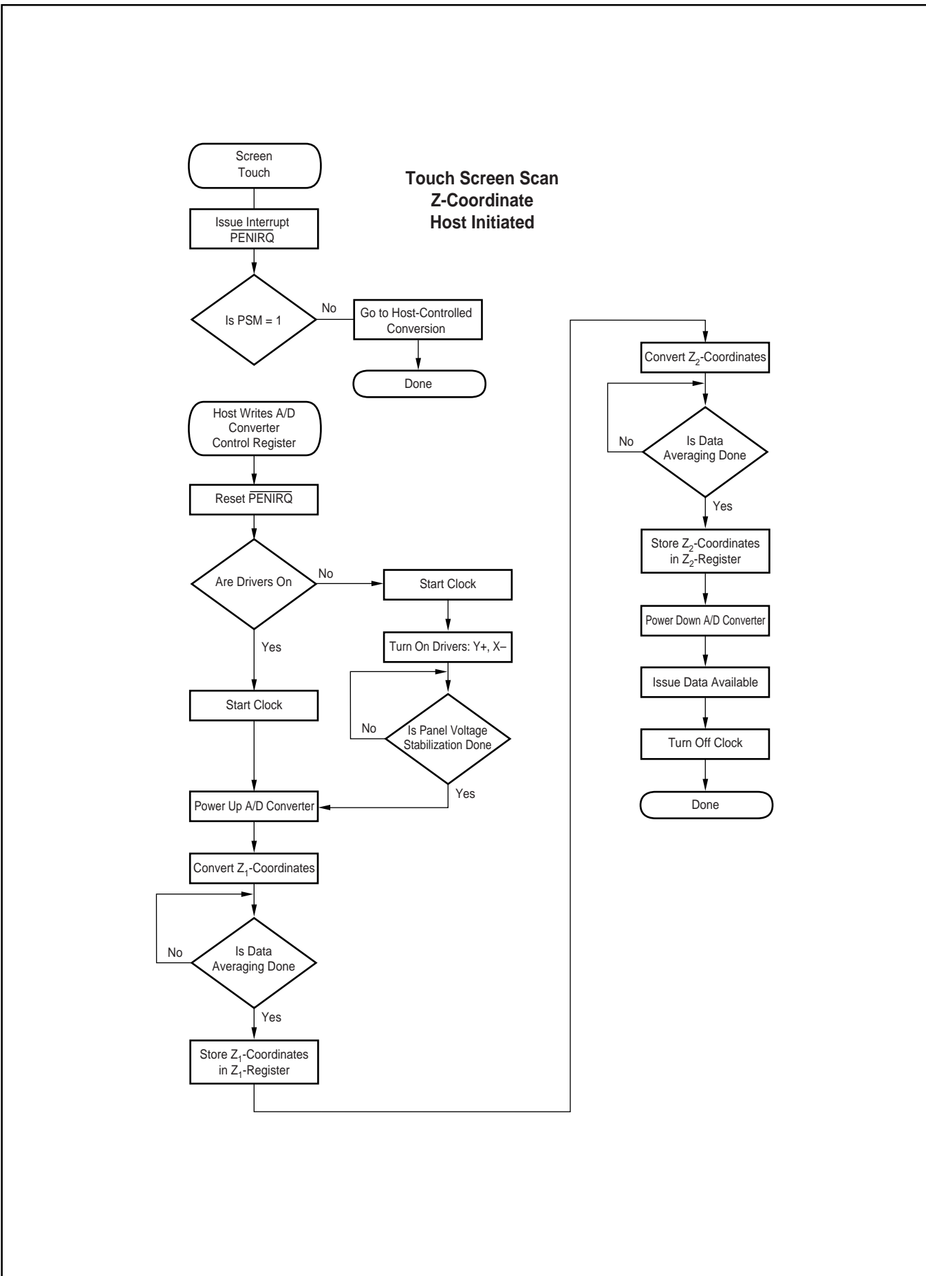
FIGURE 14. Z-Coordinate Reading Initiated by Host.
