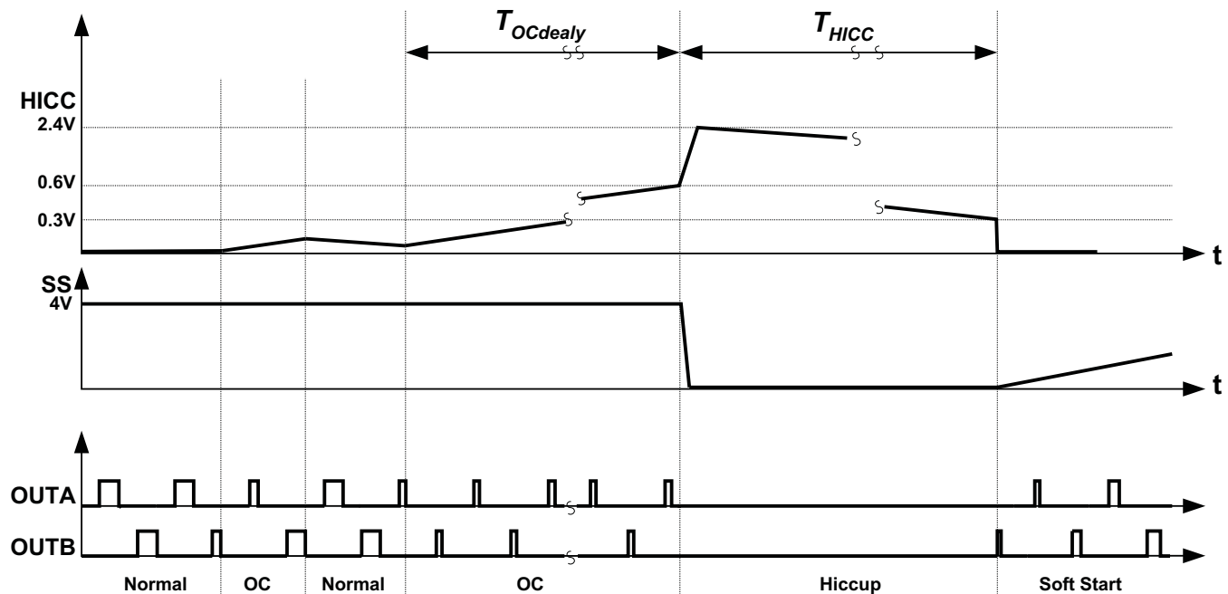
Figure 45. Cycle-by-Cycle Current Limit Delay Timer and Hiccup Restart Timer
