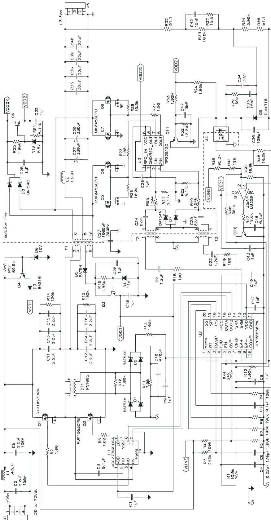
Figure 47. Schematics of Primary-Side Control Design Example
