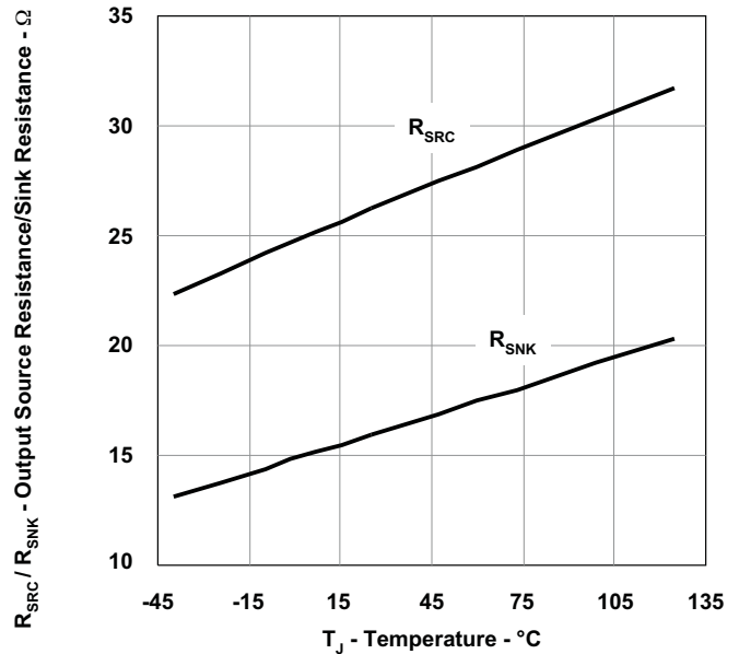
OUTPUT SOURCE RESISTANCE/SINK RESISTANCE vs TEMPERATURE
