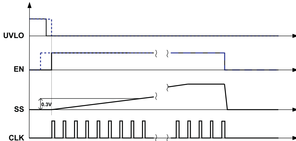
Figure 3. Level Enable at EN pin
