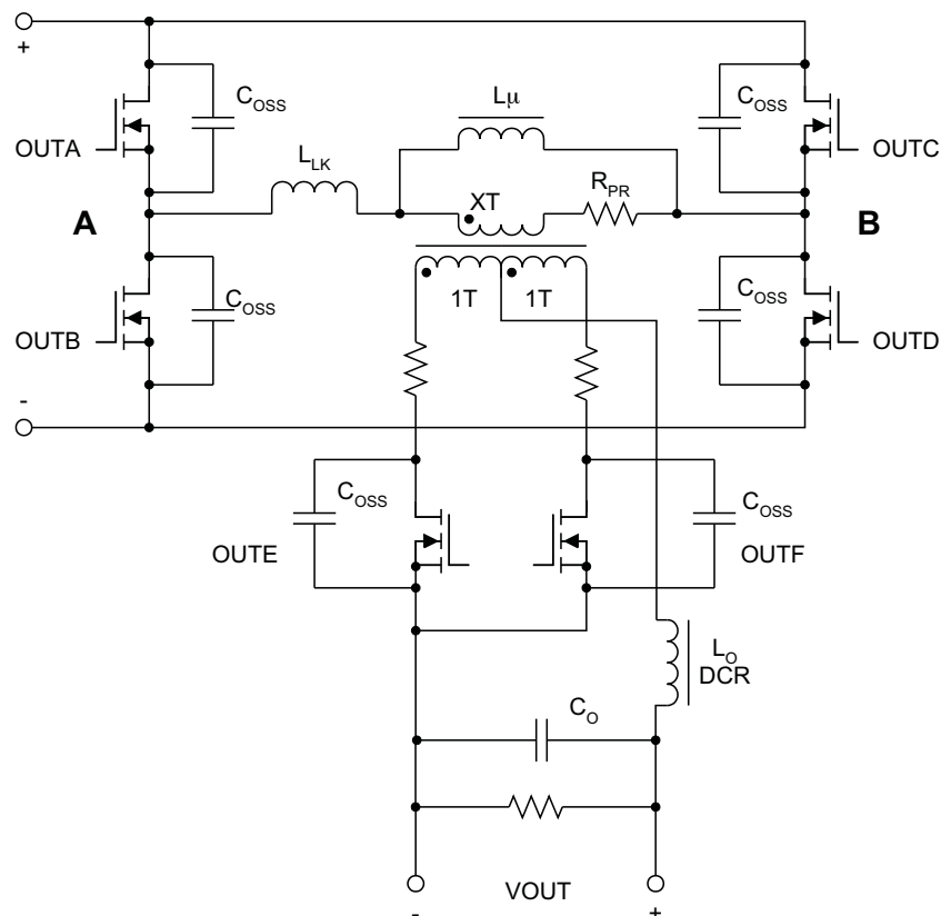
Figure 20. Power Stage
