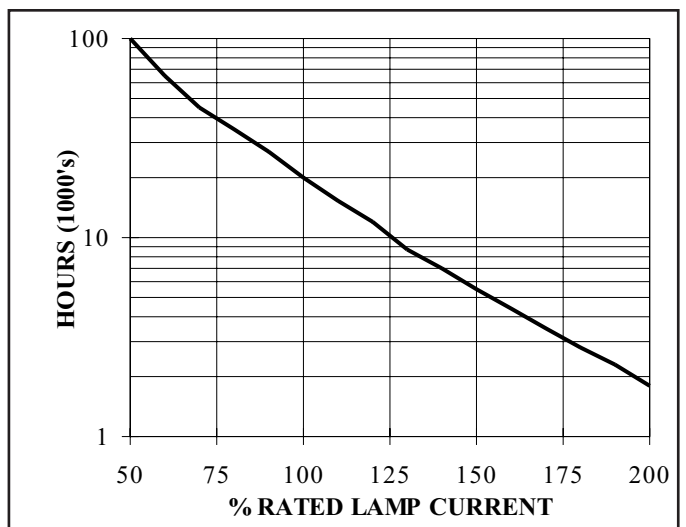
Figure 16. Lamp life versus current.
