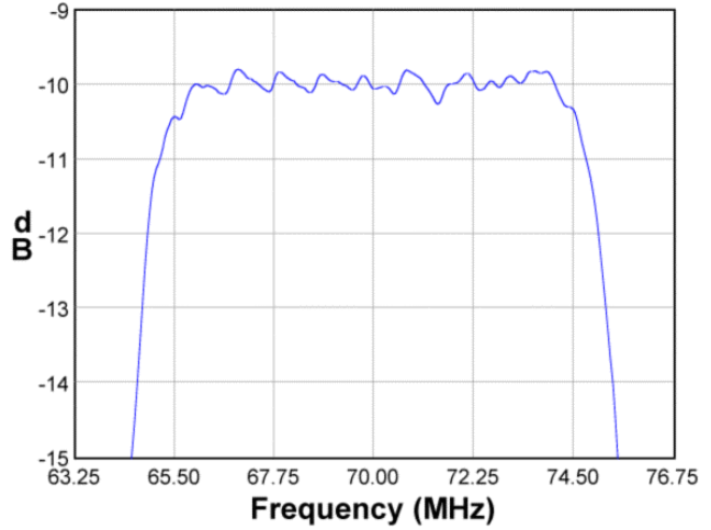
Passband Response
