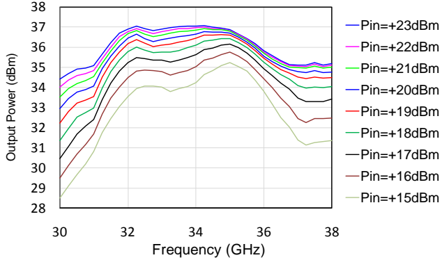
Output Power vs. Freq. vs. Input Power Vd = 6 V, Id = 2.1 A, Vg = -0.60 V Typical, +25°C
