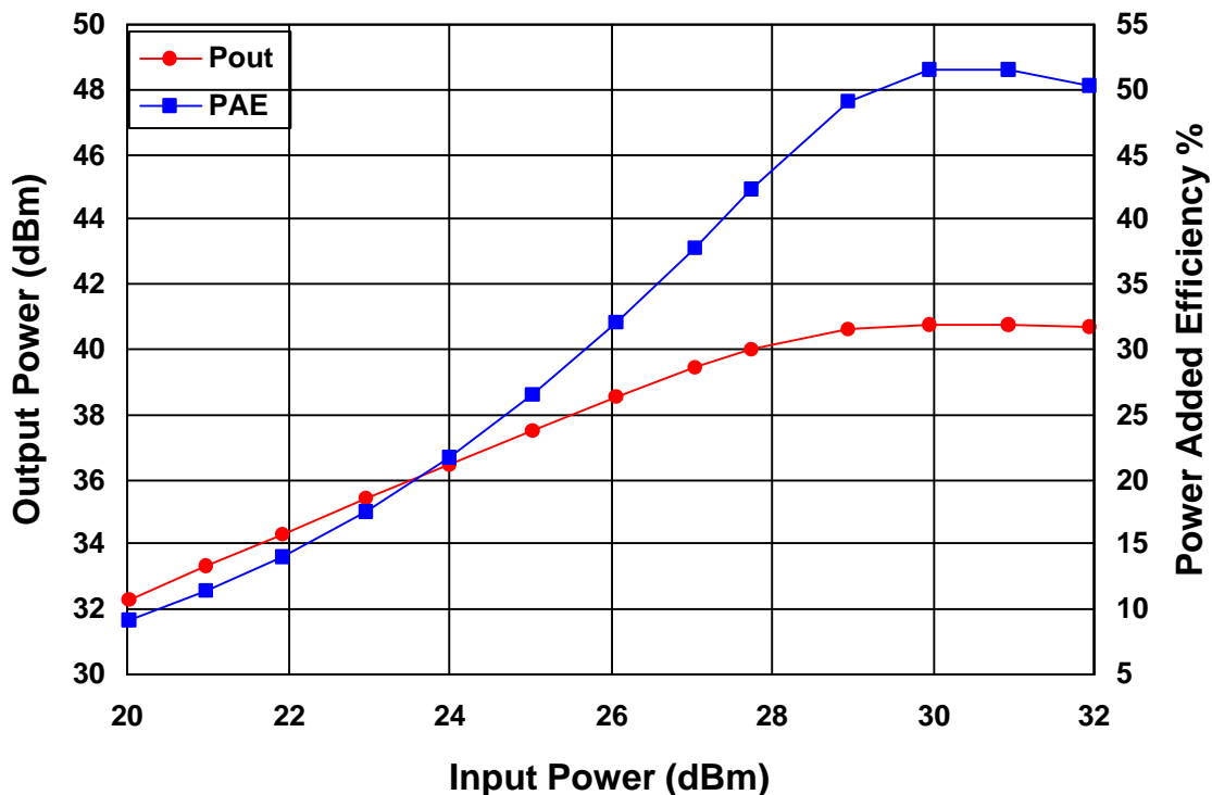
TGF4124 RF Performance at F = 2.3 \text{ GHz} V_d = 8.0 \text{ V} , V_g = -1.1 \text{ V} , I_q = 2.17 \text{ A} and T_A = 25^\circ\text{C}
