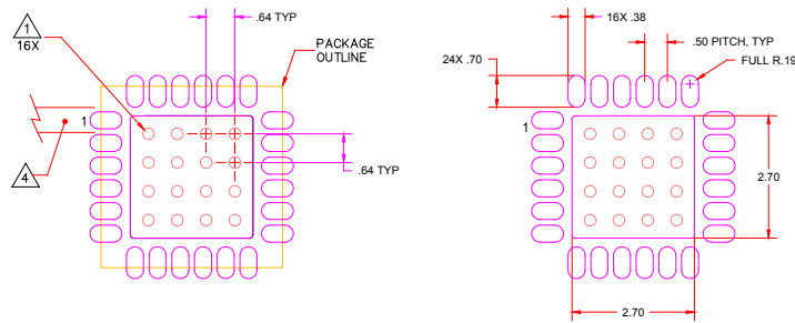
COMPONENT SIDE
