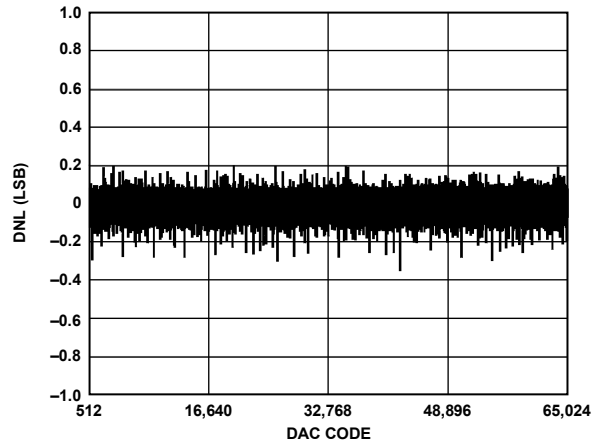
Figure 9. AD5065 DNL
