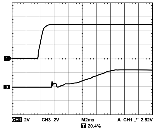
Figure 23. Power-On Reset to Midscale
