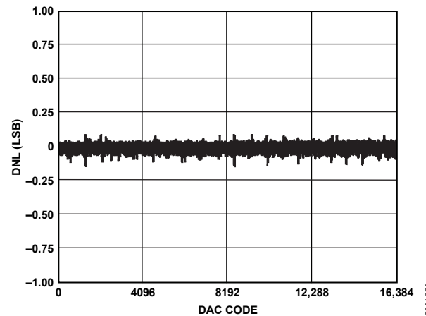
Figure 11. AD5025 DNL
