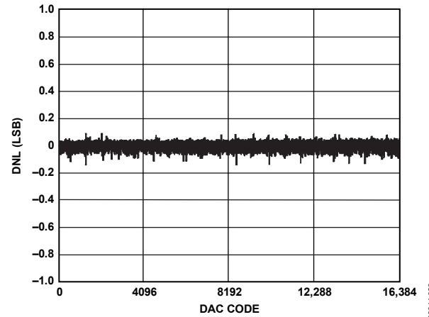
Figure 10. AD5045 DNL
