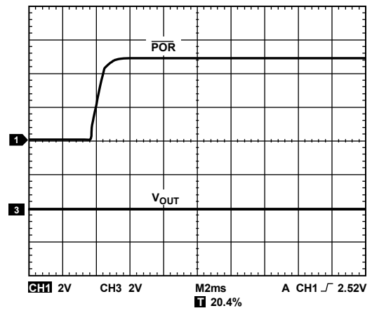
Figure 22. Power-On Reset to 0 V
