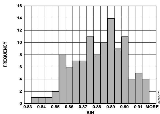
Figure 38. I_{DD} Histogram V_{DD} = 3.0V
