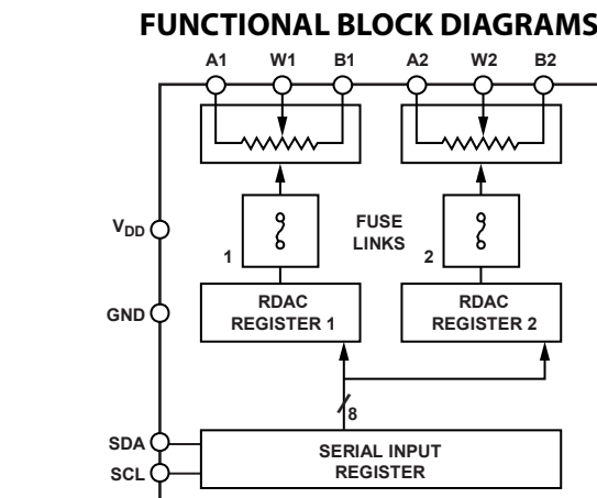
Figure 1. AD5172 Functional Block Diagram
