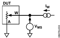
Figure 38. Resistor Position Nonlinearity (Rheostat Operation; R-INL, R-DNL)
