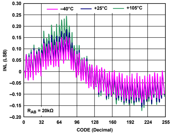
Figure 20. R-INL in R-Perf Mode vs. Code vs. Temperature (AD5291)
