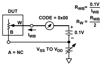
Figure 60. Wiper Resistance
