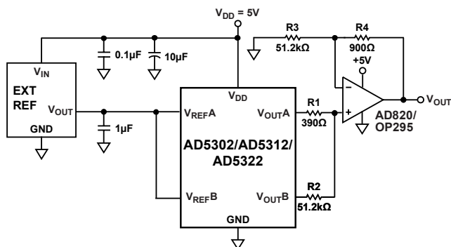
Figure 44. Coarse/Fine Adjustment
