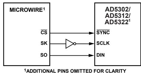
Figure 37. AD5302/AD5312/AD5322 to MICROWIRE Interface
