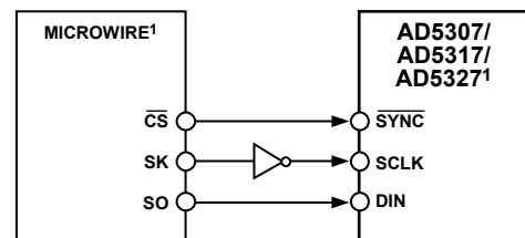
Figure 40. MICROWIRE-to-AD5307/AD5317/AD5327 Interface
