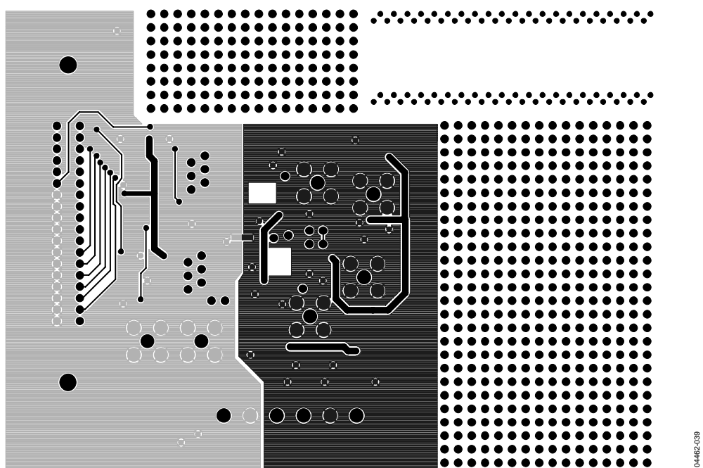
Figure 50. Solder-Side Artwork
