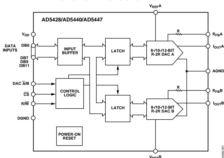
Figure 1. AD5428/AD5440/AD5447
