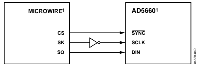
Figure 48. AD5660-to-MICROWIRE Interface
