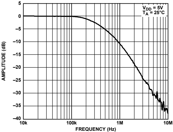
Figure 49. Multiplying Bandwidth
