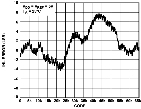
Figure 6. AD5667R INL, External Reference
