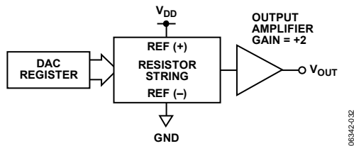
Figure 52. DAC Architecture
