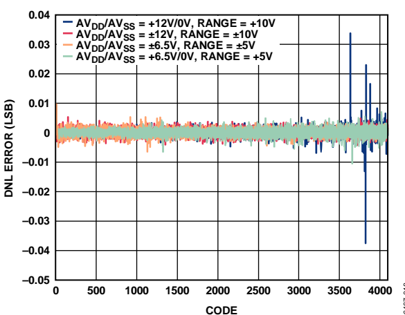
Figure 11. AD5722 Differential Nonlinearity Error vs. Code
