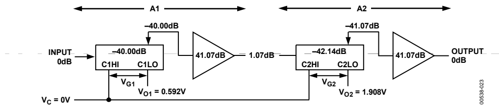
Figure 23. AD600 Gain Control Input Calculations for Sequential Control Operation (A)
