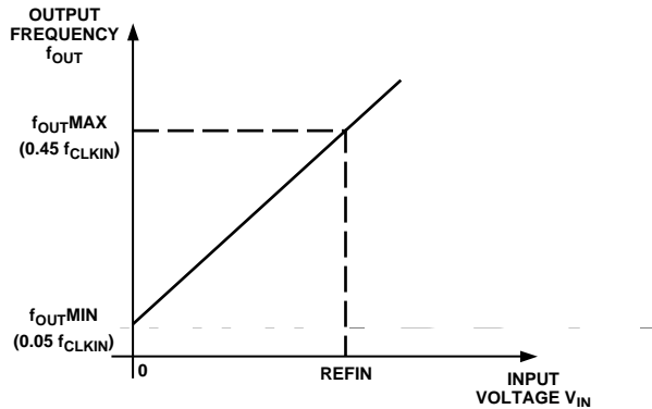
Figure 3. AD7741 Transfer Characteristic for Input Range from 0 to V_{REF}
