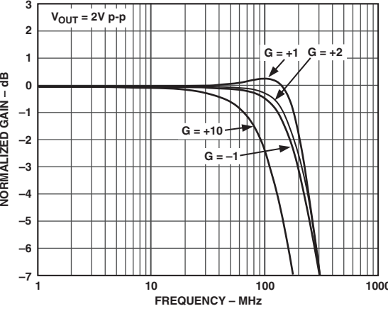
TPC 9. Large Signal Frequency Response for Various Gains
