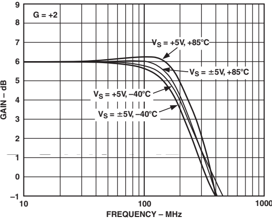
TPC 11. Small Signal Frequency Response over Temperature, V_S = +5\text{ V}, \pm 5\text{ V}
