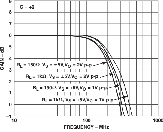
TPC 12. Large Signal Frequency Response for V_S and R_{LOAD}
