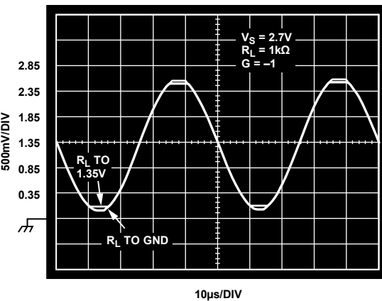
Figure 40. Output Swing
