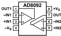
Figure 3. MSOP-8 and SOIC-8 (RM-8, R-8)
