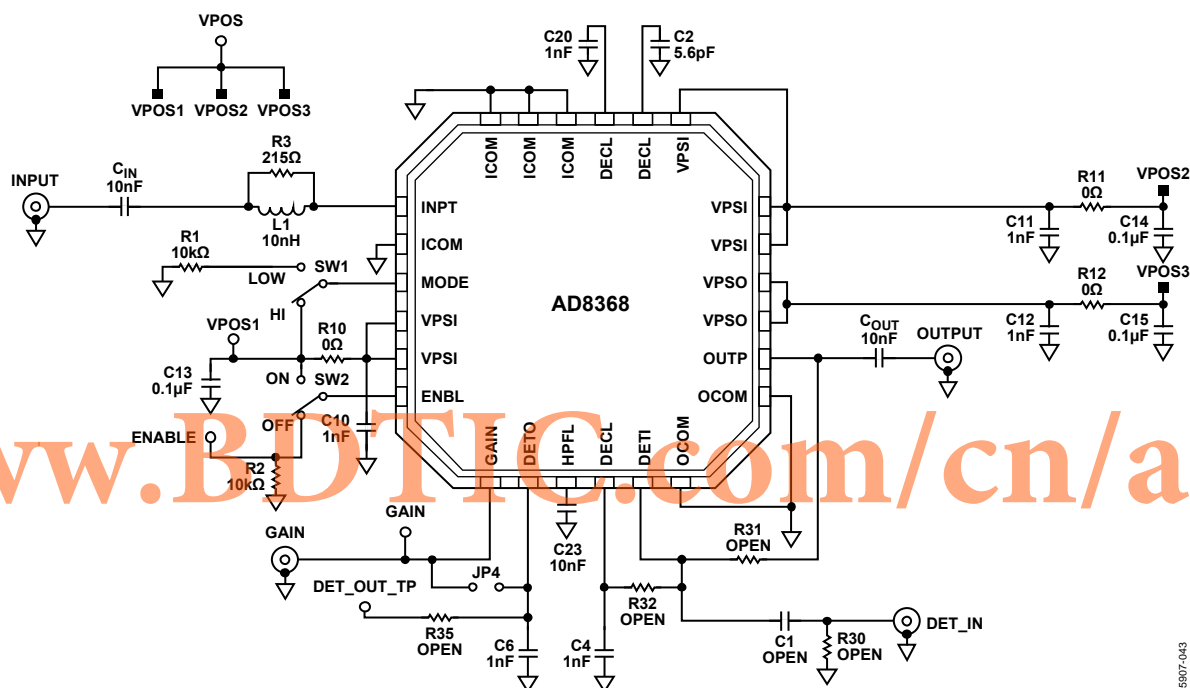
Figure 40. Evaluation Board
