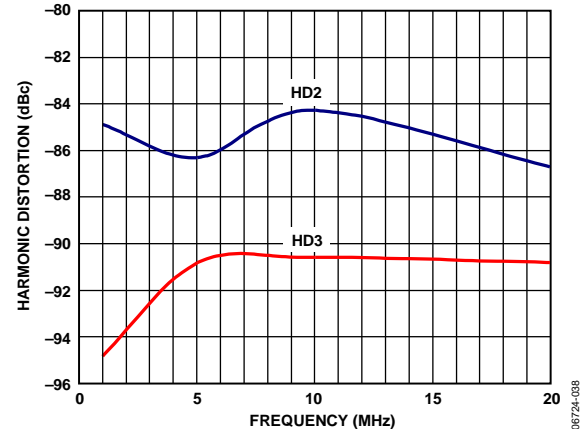
Figure 37. Harmonic Distortion vs. Frequency Using Resistive Pull-Ups
