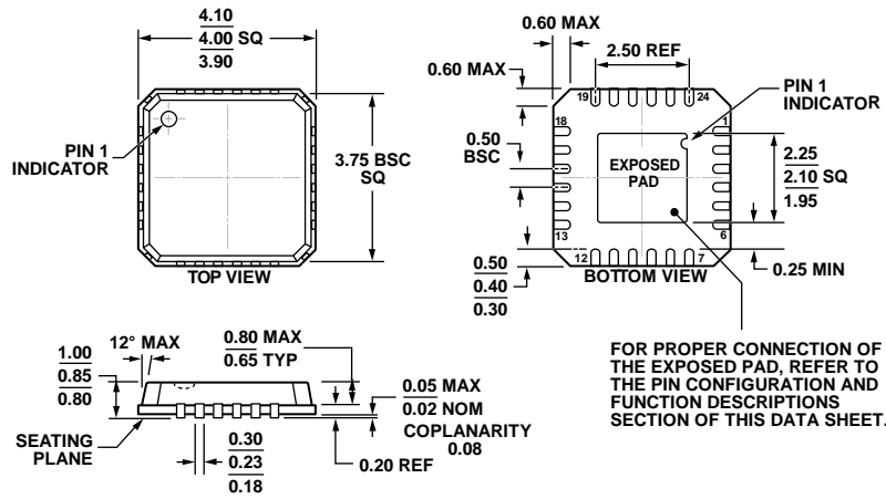
Figure 51. 24-Lead Lead Frame Chip Scale Package [LFCSP_VQ] 4 mm × 4 mm Body, Very Thin Quad (CP-24-1) Dimensions shown in millimeters
