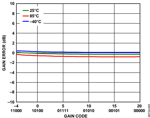
Figure 6. Gain Error over Temperature at 140 MHz
