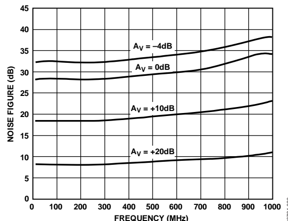
Figure 21. NF vs. Frequency
