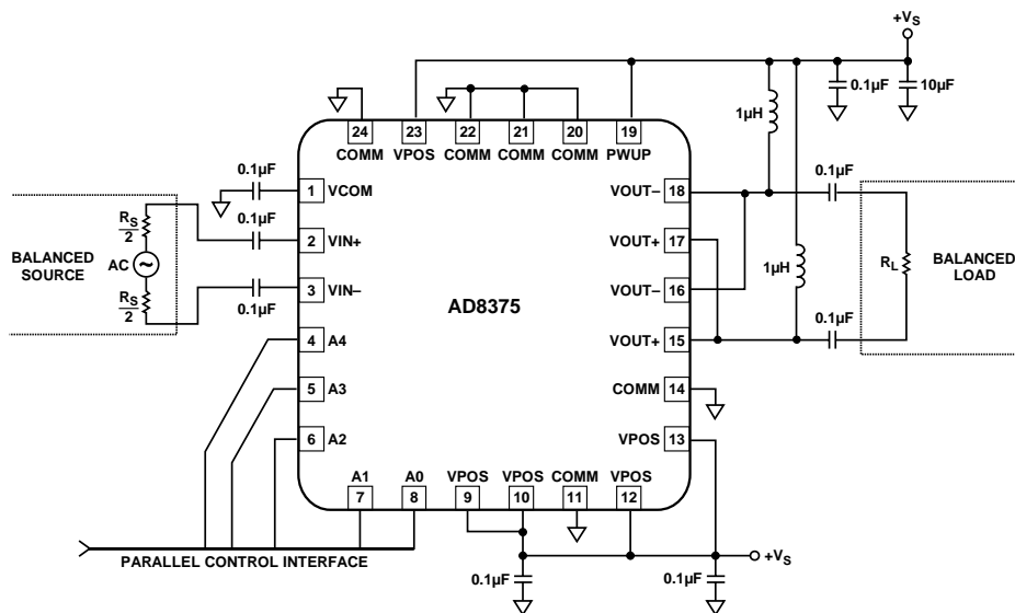
Figure 35. Basic Connections
