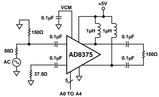
Figure 33. Single-Ended-to-Differential Conversion
