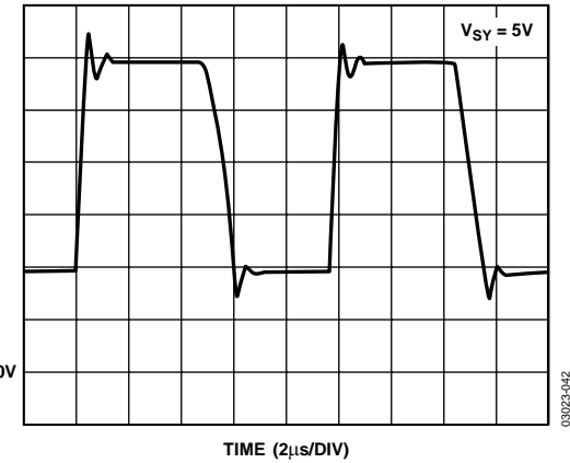
Figure 43. Gain-of-Two Inverter Response to 20 mV Step, Centered 20 mV below Ground
