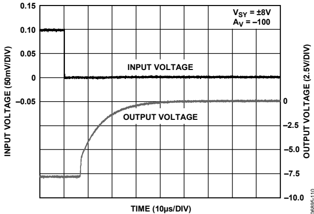
Figure 46. Positive Input Overload Recovery for the AD8638
